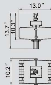
Model:HLI-1000GBR Material:Die-Casting Aluminium
