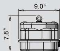
Model:HLI-400GB Material:Die-Casting Aluminium
