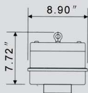
Model:HLI-400GB-A Material:Die-Casting Aluminium
