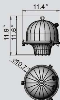
Model:HLI-400GB-C Material:Die-Casting Aluminium
