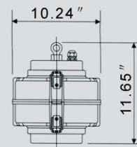
Model:HLI-400GB-D Material:Die-Casting Aluminium
